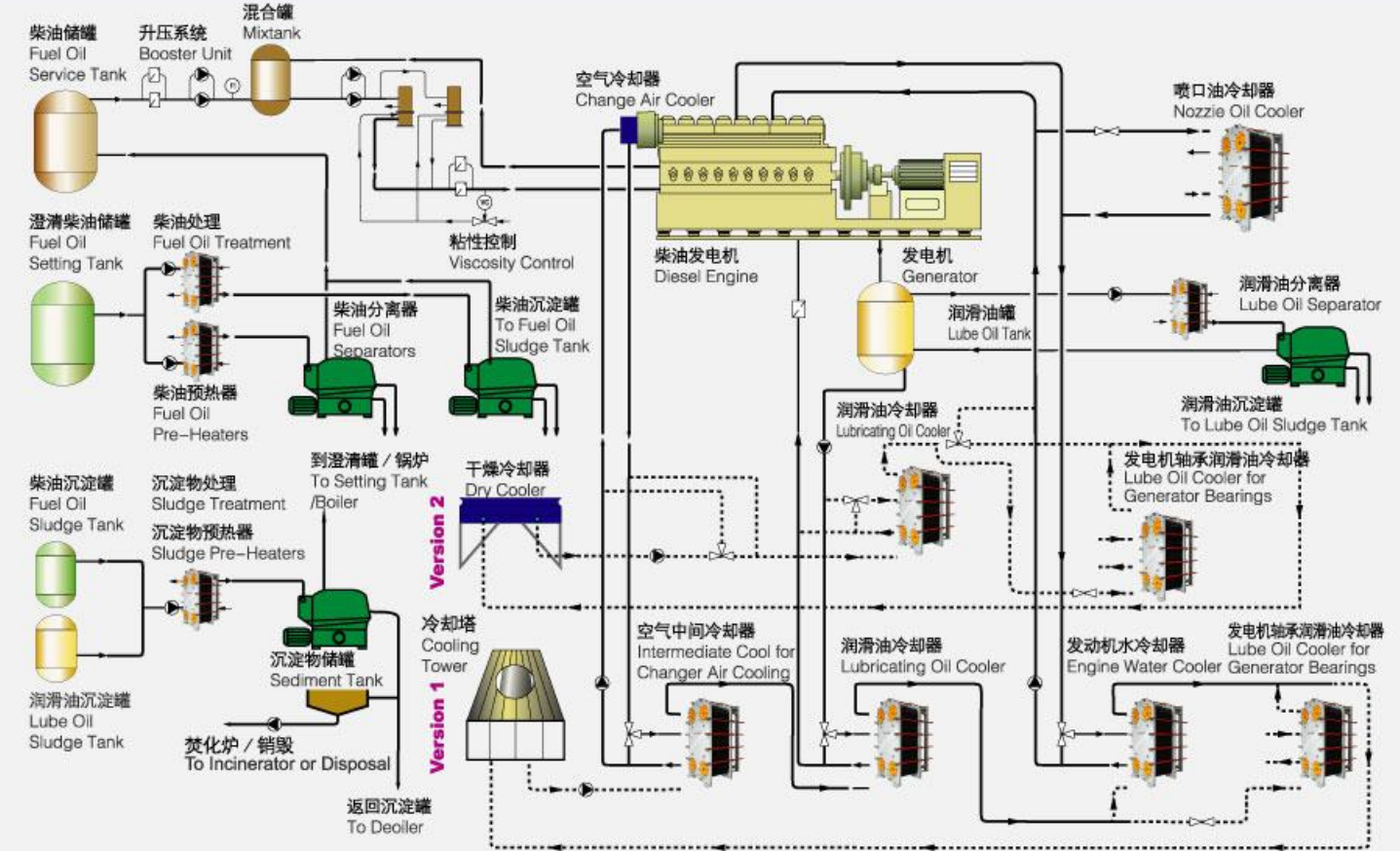
板式换热器在电厂柴油机冷却系统的应用 (原理图) Plate Heat Exchangers Used in Cooling System of Diesel Engines in Power Plants (Schematic Diagram)
